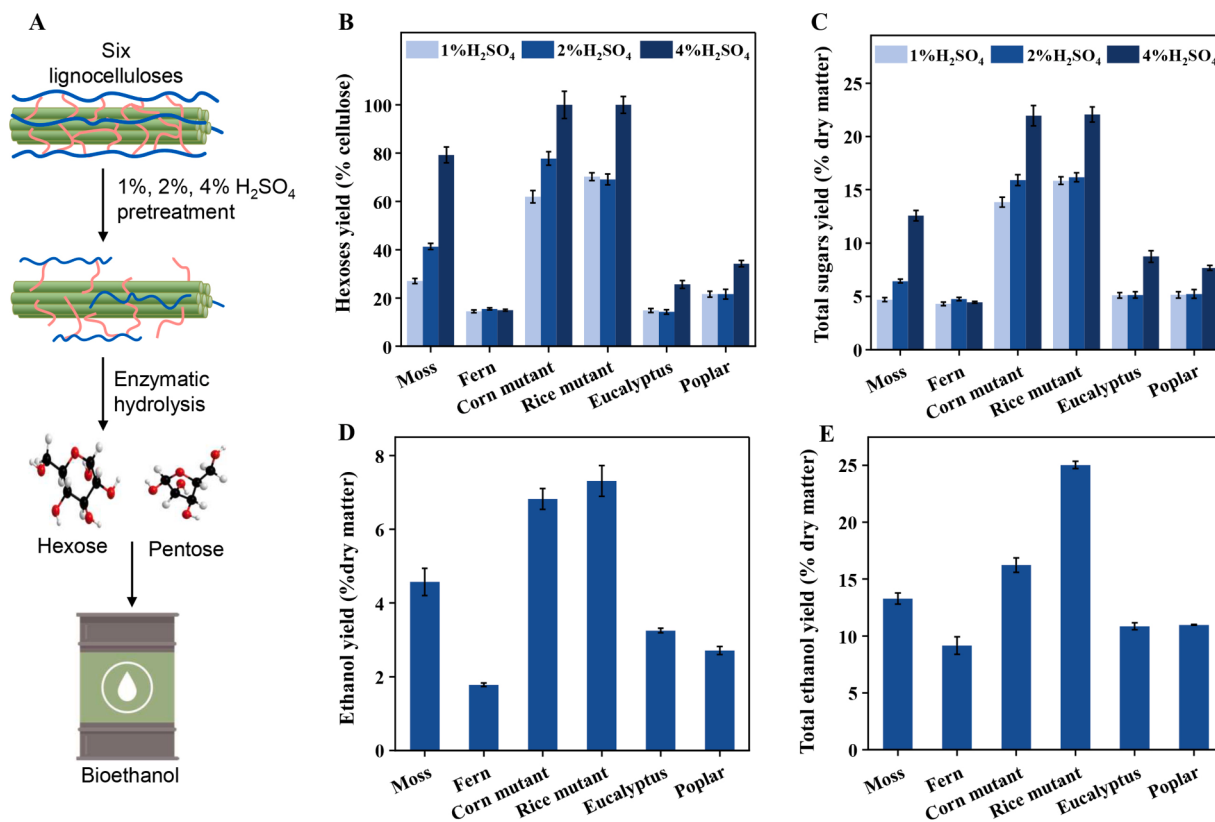
Fig. 2. Hexoses and bioethanol yields from enzymatic hydrolyses of six plant species after H_2SO_4 pretreatment at different concentrations. (A) Experimental flow chart for biomass saccharification and bioethanol fermentation; (B) Hexoses yield; (C) Total sugars (hexoses and pentoses) yield from enzymatic hydrolysis after pretreatment; (D) Ethanol yield by real yeast fermentation with hexoses released from enzymatic hydrolysis after 4% H_2SO_4 pretreatment; (E) Total ethanol yield by yeast fermentation with total sugars released from both enzymatic hydrolysis and 4% H_2SO_4 pretreatment with xylose-ethanol conversion in theory; Bar as means \pm SD ( n = 3 ).
