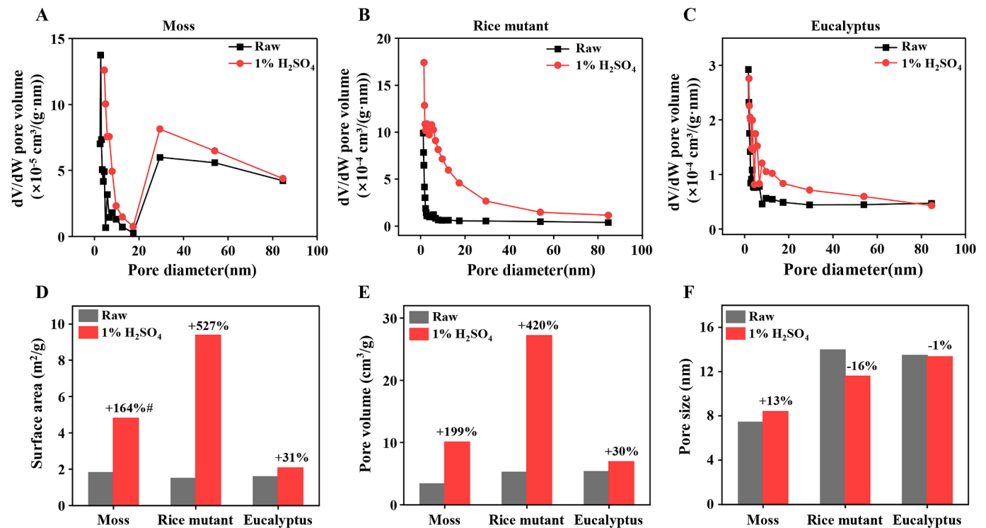
Fig. 4. Brunauer-Emmett-Teller (BET) analysis of lignocellulose porosity of three representative plant species after 1% H 2 SO 4 pretreatment. (A-C) Barret-Joyner-Halenda (BJH) adsorption micropore distribution; (D) BET surface area; (E) Pore volume; (F) Pore size; # As increased (+) or decreased (−) percentage of the acid-pretreated lignocellulose relative to its raw material.
